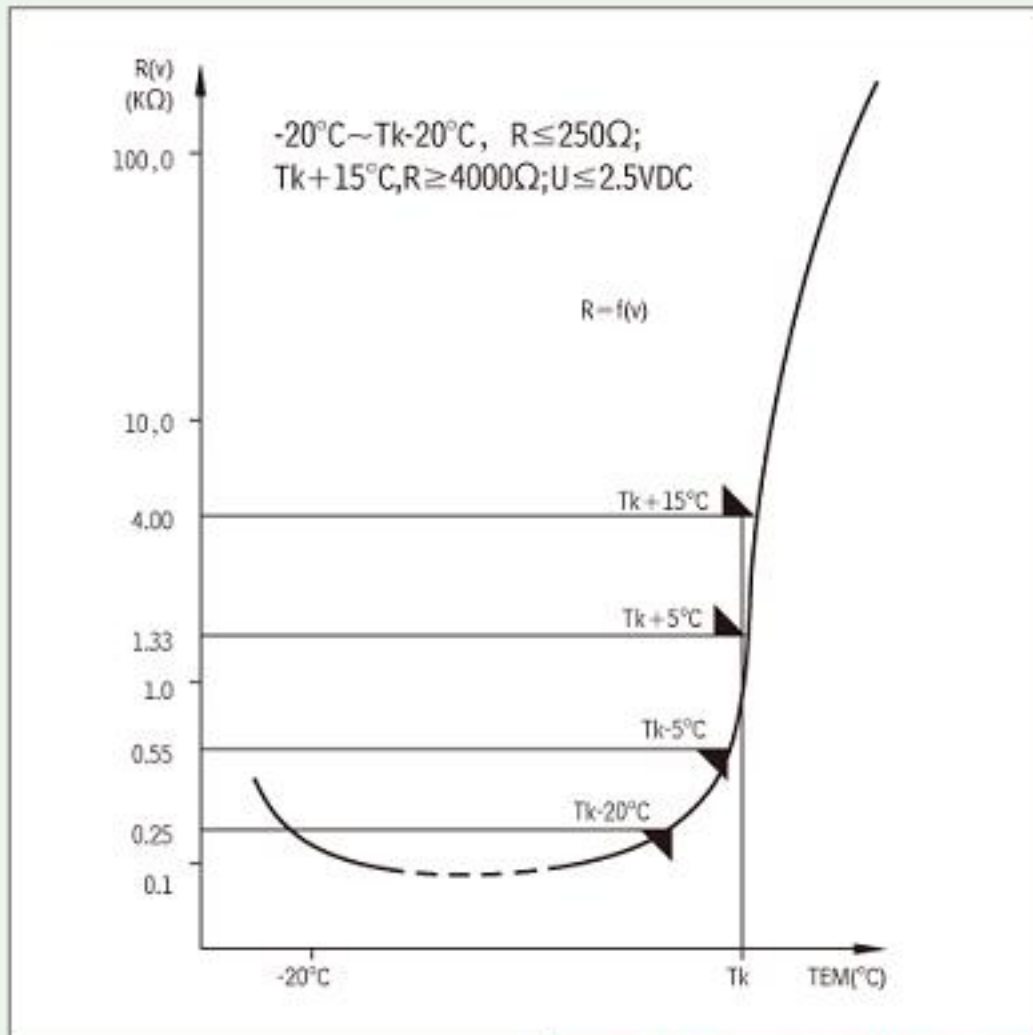
PTC characteristic curve acc. to DIN 44081/082
